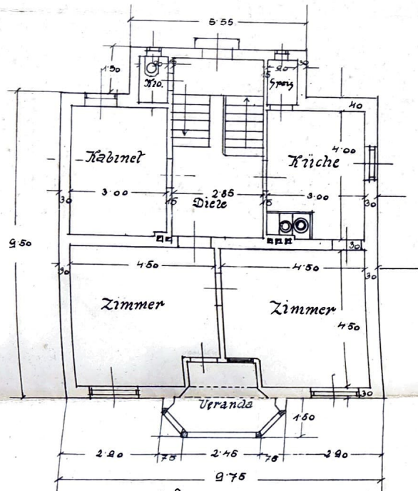
Erdgeschoss.
