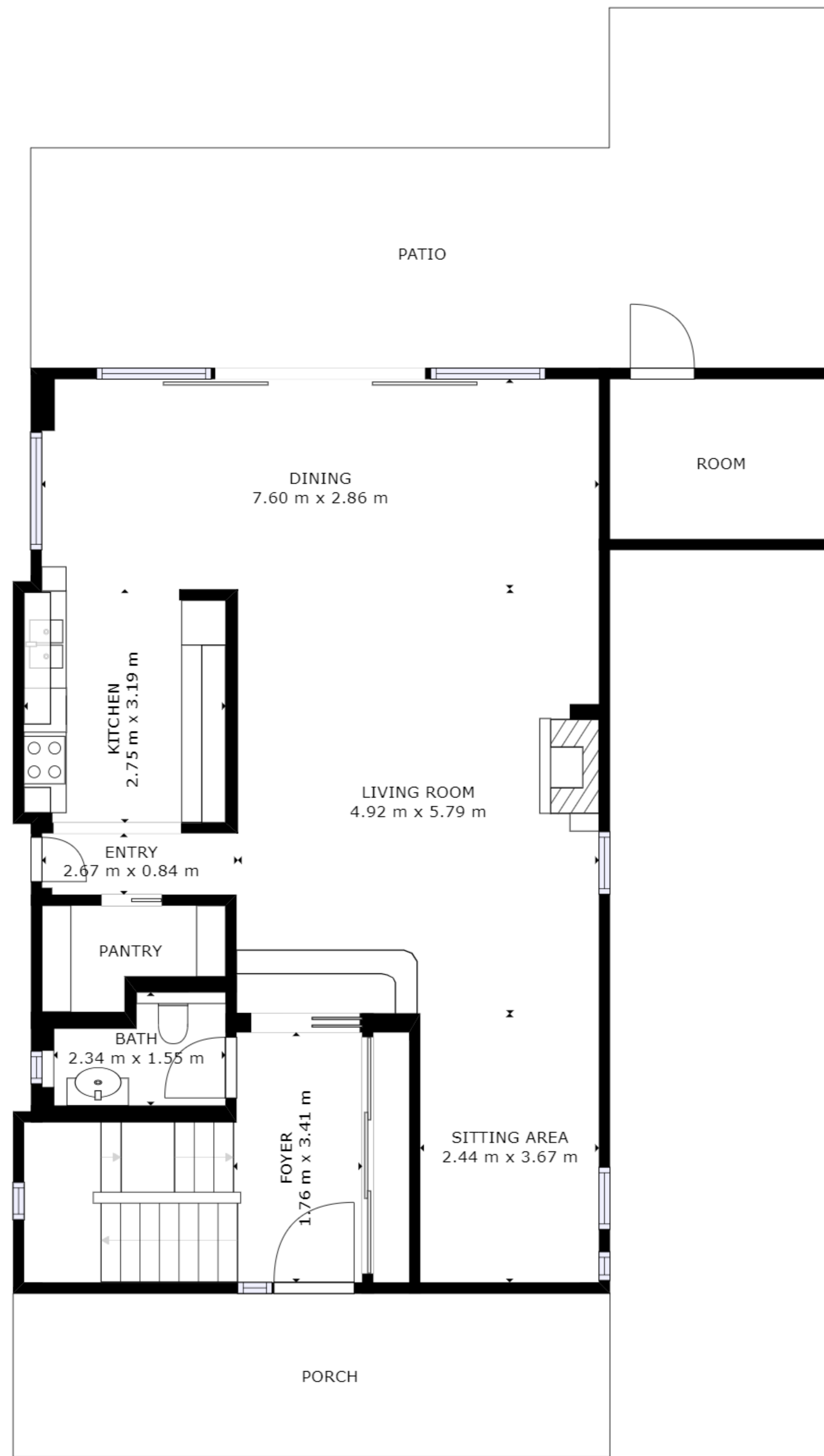
FLOOR 2
